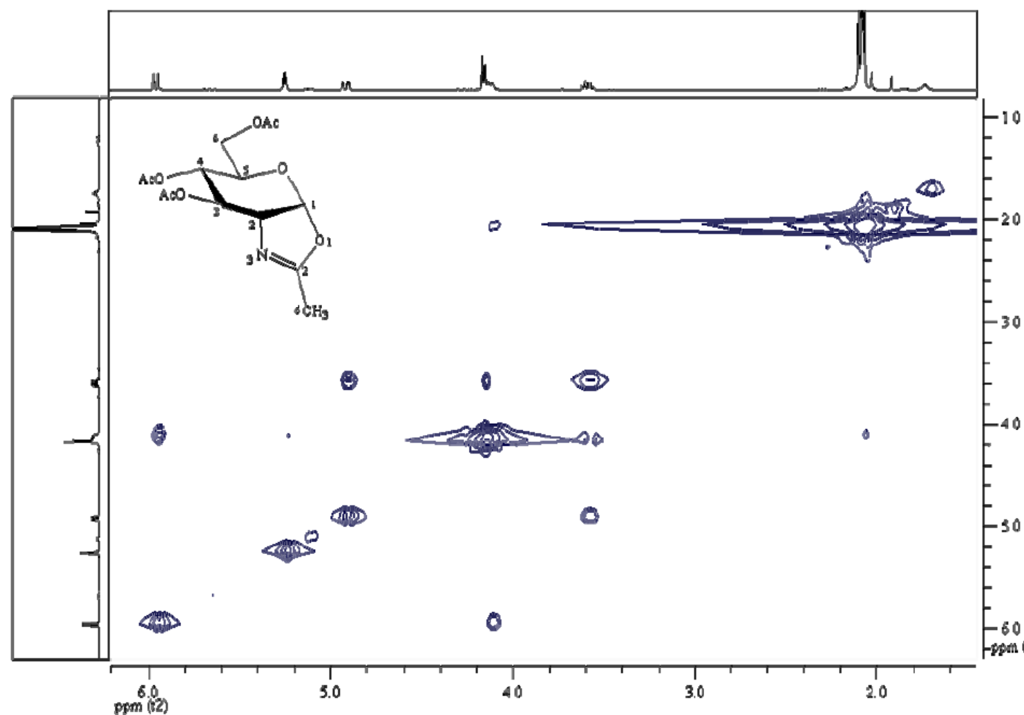
H,H-COSY of an oxazoline-glucose
