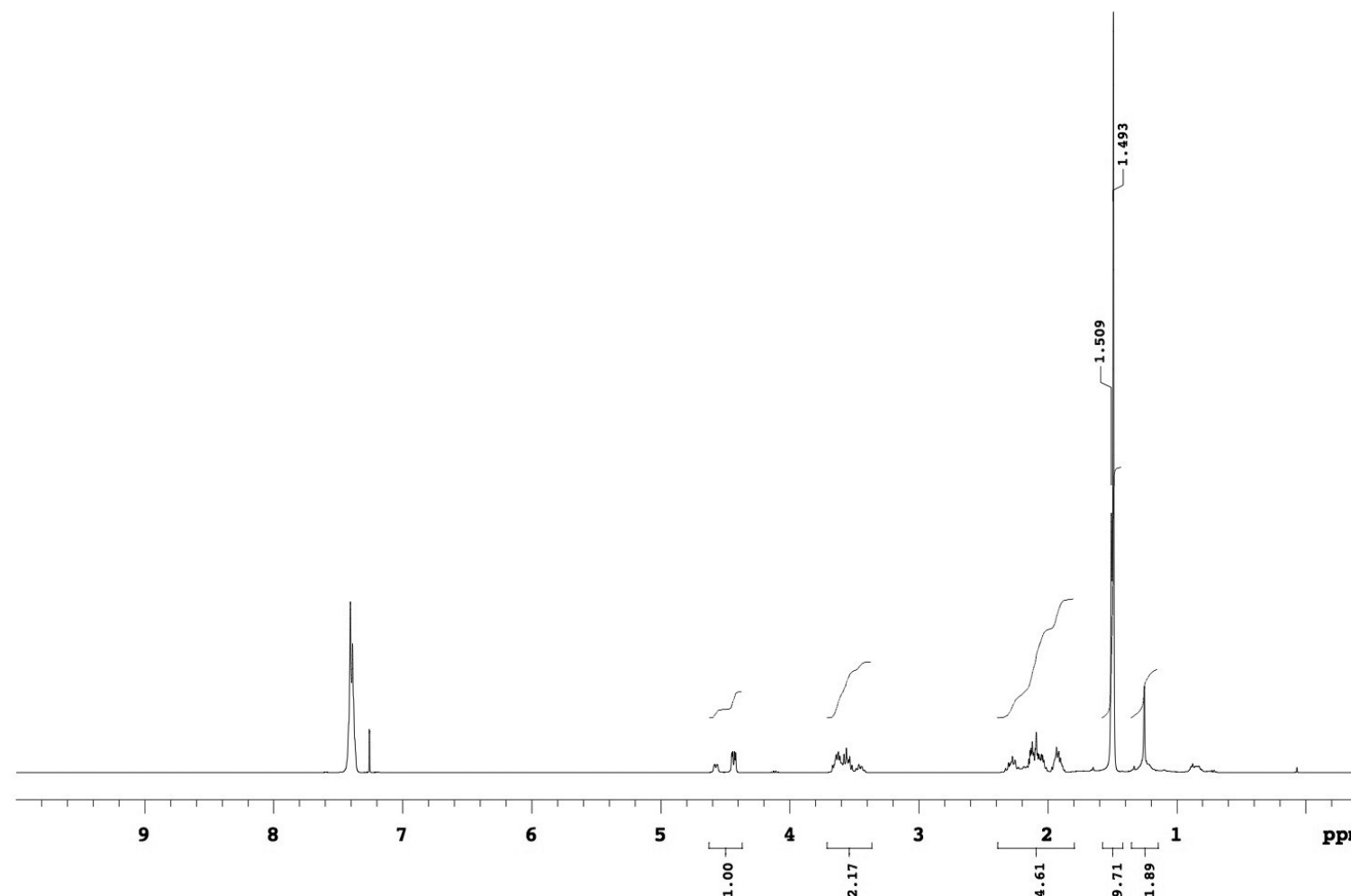
Thiophenyl-Boc-N-proline spectrum
