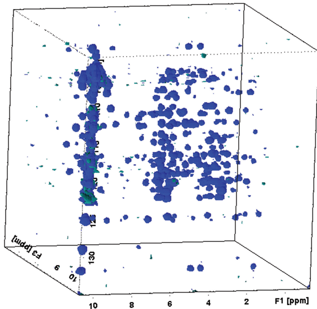
3D ^{13}\text{C} NOESY of a protein
