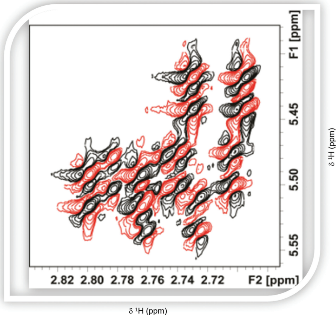
2D COSY spectrum of a flavonoid mixture
