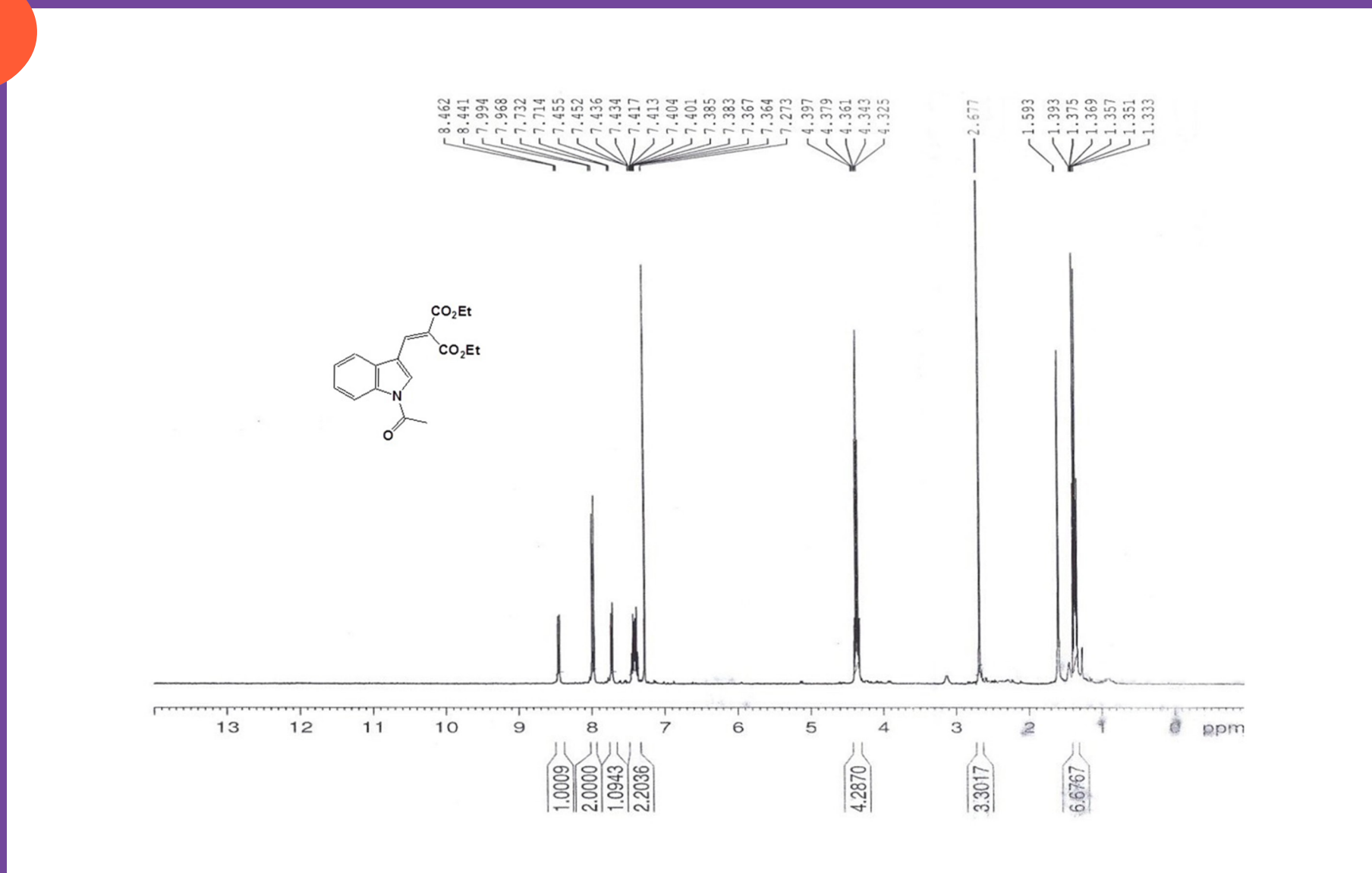
Diethyl 2-((1-acetyl-1H-indol-3-yl)methylene)malonate
