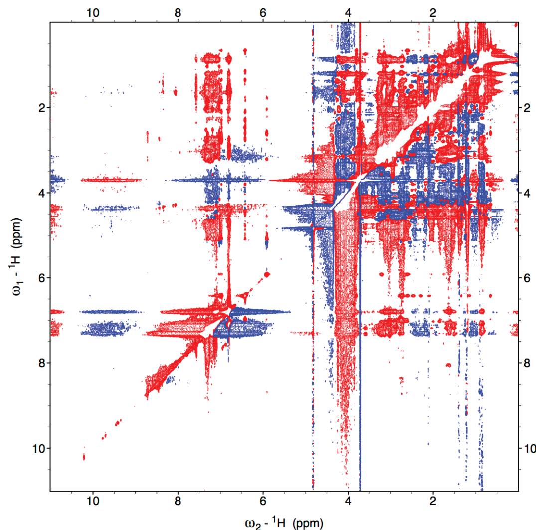
2D NOESY spectrum using MCR-LDL \alpha protein
