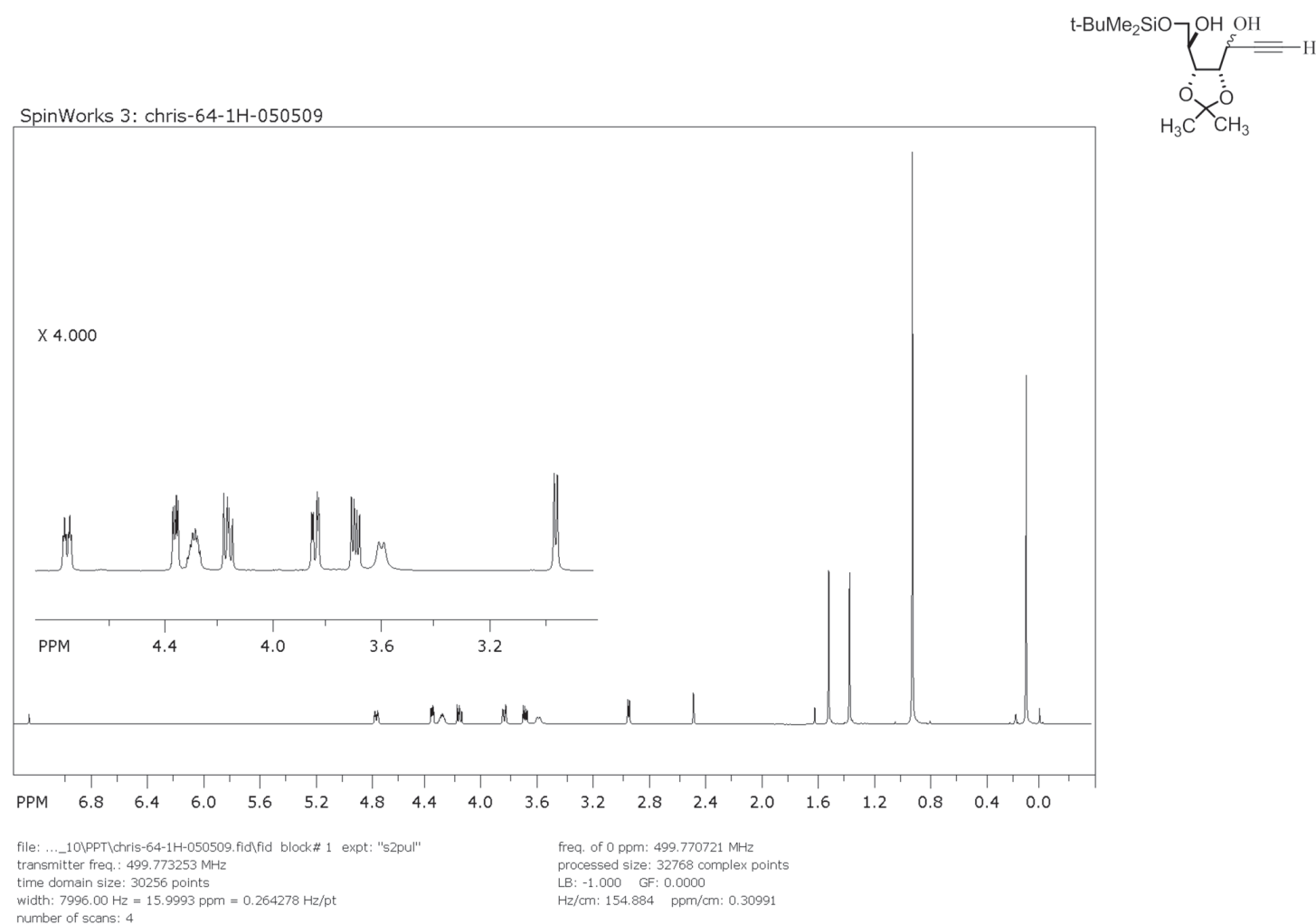
Diol 63 Dilute Sample
