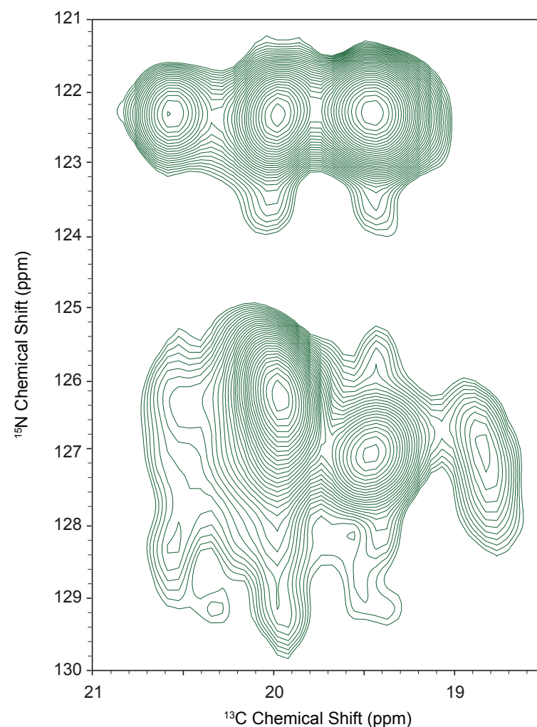
^{13}\text{C} - ^{15}\text{N} TEDOR spectrum of human prion 23-144 fibrils
